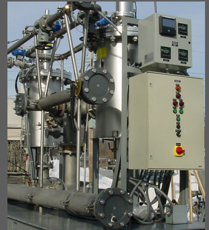
U.S. Navy seawater pump/filter process systems
